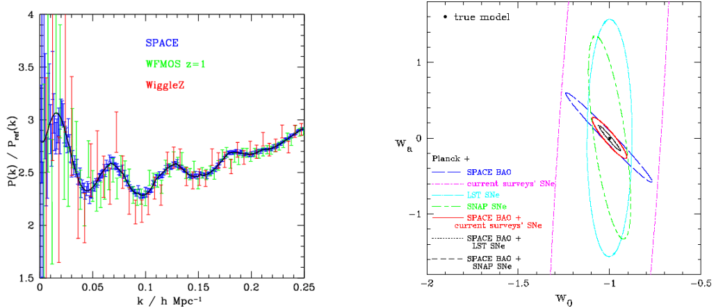
Fig. 1. – Left : the appearance of BAO in selected ongoing and future surveys. The measured power spectrum has been divided by a featureless reference spectrum to show the BAO more clearly. WiggleZ is an on-going survey of emission line selected galaxies at z \sim 0.7 . WFMOS is a spectroscopic, ground-based survey proposed for Subaru. The blue points show the measurements expected from the full survey volume of SPACE. The black solid line represents the theoretical model for the BAO. The high frequency sampling and small errors of P(k) from SPACE mean that we will achieve the definitive measurement of the BAO. The statistical power of the SPACE BAO measurement is around an order of magnitude better than that expected from WFMOS. Right : The joint 68% confidence interval constraints on the dark energy equation of state parameter ( w_0 ) and its evolution with redshift ( w_a ). Several datasets can be combined to improve the constraints. SPACE will dramatically improve our knowledge of w_0 and w_a .
